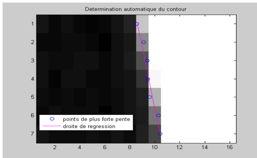
fig. 13 - sub pixel location of the edge location and interpolation.
