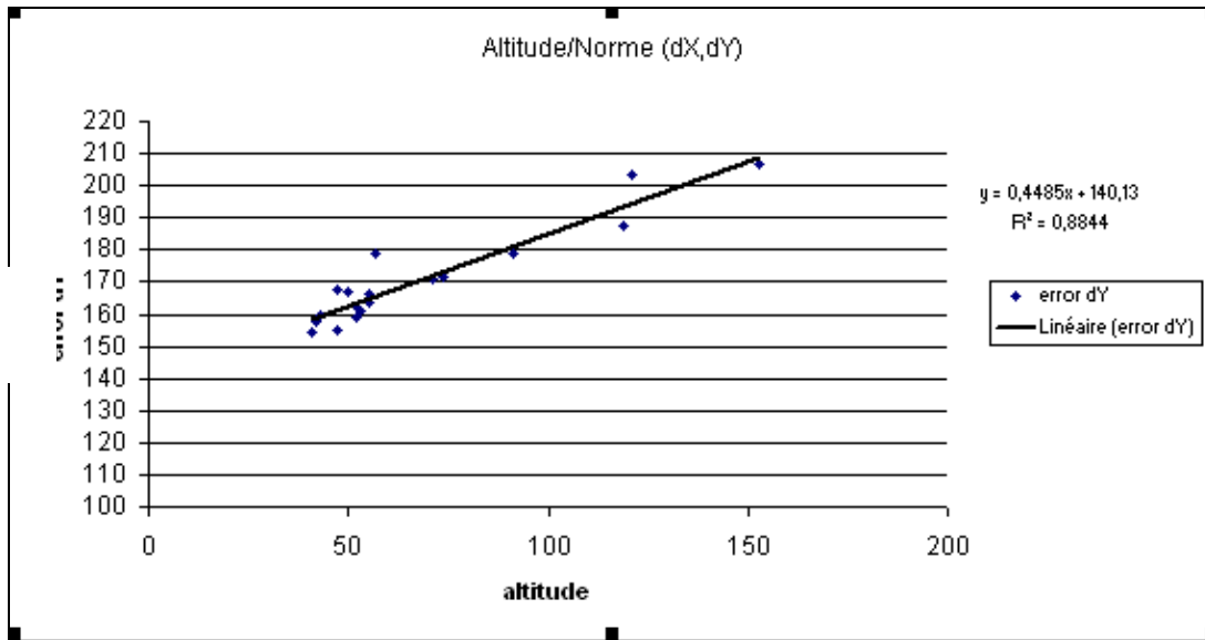
fig. 6 - Trend analysis, norm of displacement errors along with altitude, ALPSMN065....
